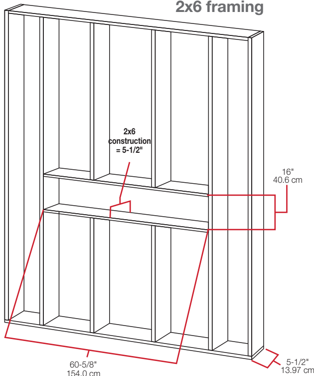
2x6 framing
