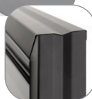
60" IgniteXL Trim Kit (XLFTRIM60) Allows installation of IgniteXL in 2"x4" wall construction. 62-3/4" x 18-1/4" x 1-7/8" (159.4 cm x 46.2 cm x 4.5 cm)
